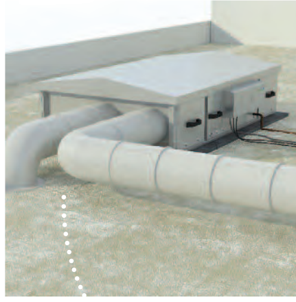
◀ (Model: XBOXER XBC45-H-NTWP). External roof mounted heat recovery unit fitted with external weather roof.
