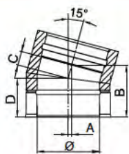
Elbow 15° / DWECO - 16
